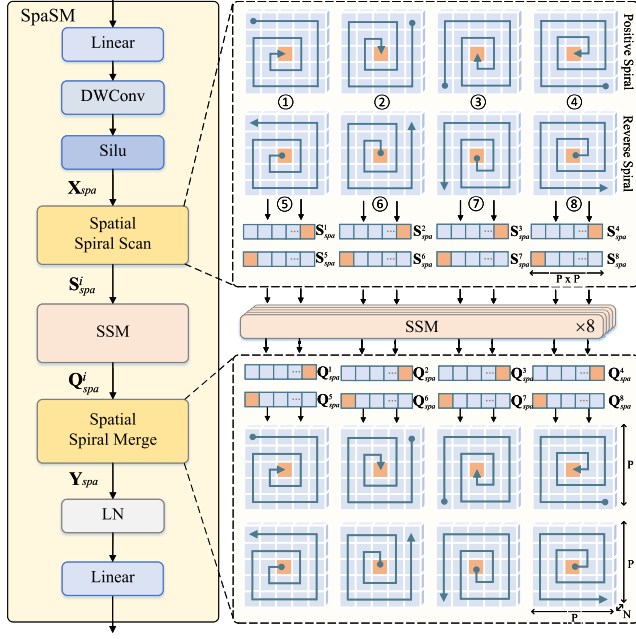
Fig. 2. Flowchart of the SpaSM. The input data is first passed through a linear layer, a DWConv layer, and a SiLU layer to obtain 2-D features \mathbf{X}_{\text{spa}} . Then, the spatial spiral scan is used to convert \mathbf{X}_{\text{spa}} into eight different 1-D spatial sequences. The spatial clues can be explored using these sequences along with eight unshared SSMs. Next, the spiral merge is used to restore the processed sequences into 2-D versions and combine them. Finally, the output of SpaSM can be obtained by passing the restored and integrated feature through an LN layer and a linear layer. ①–⑧ in the figure refer to the eight different spiral scan paths.
